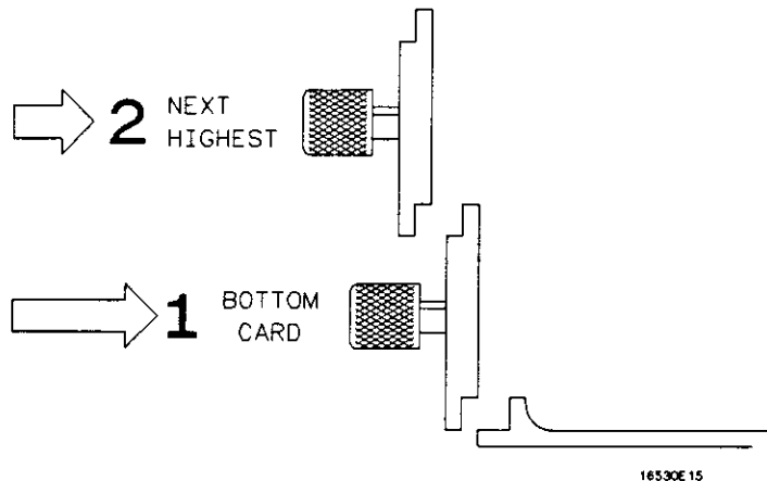
Figure F-3. Endplate Overhang
