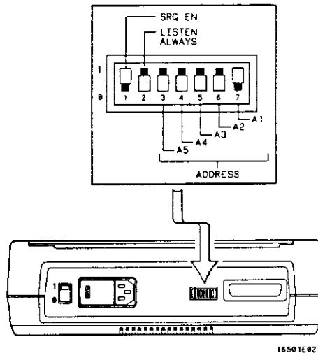
Figure 7-2. Configuration Switches for the HP ThinkJet Printer
