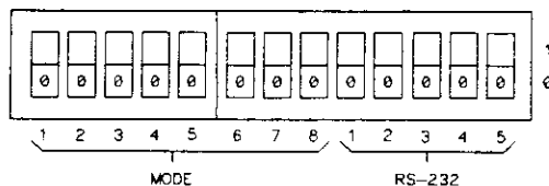
Figure 7-6. Switch Configuration for HP ThinkJet Printers
